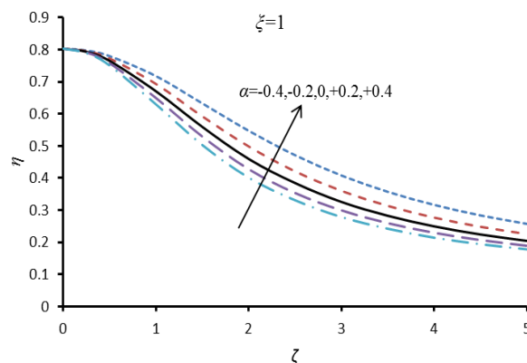
Fig. 5 Efficiency of porous fin for different values of convection and \alpha parameter
