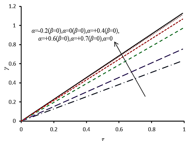
Fig. 8 Thermo-geometric fin parameter dependency of the ratio of porous fin to solid fin heat transfer rate for different values of \alpha and \beta parameters
