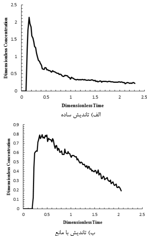
Fig. 5 Residence time diagrams for different tundishes
