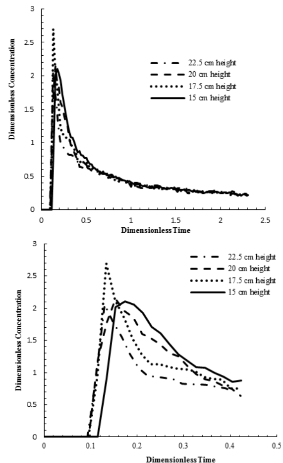
Fig. 8 Comparison of residence time diagrams for single tundish with different water heights
