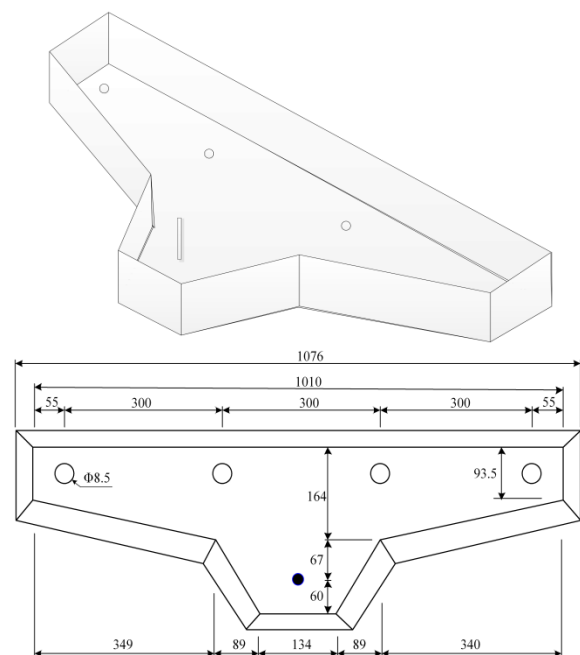
Fig. 1 Geometry and physical dimensions of the model tundish
