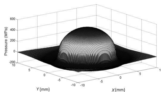
Fig. 12 Hertz pressure distribution in and out of the contact area
