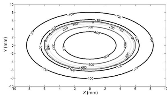
Fig. 11 Hertz pressure contour in and out of the contact area (MPa)
