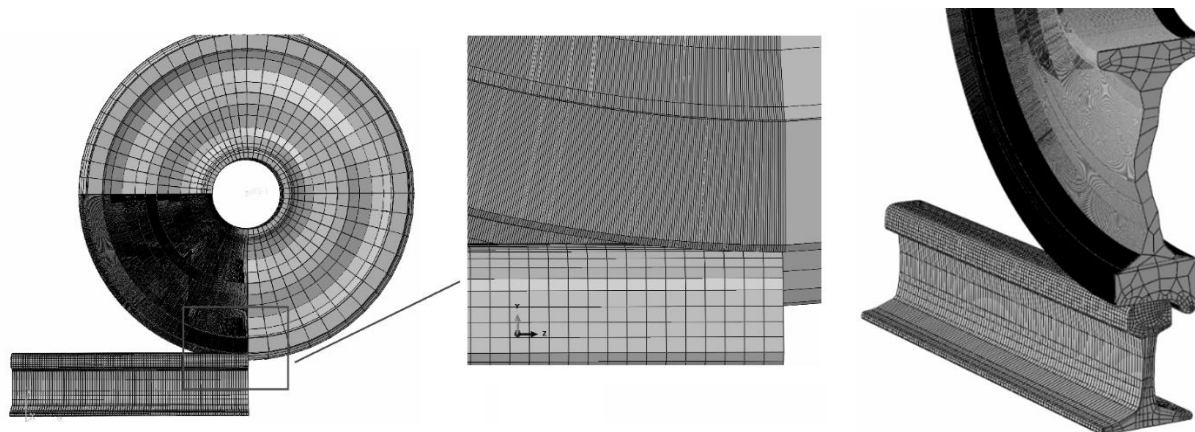
Fig. 9 Discretization of the wheel-rail contact
