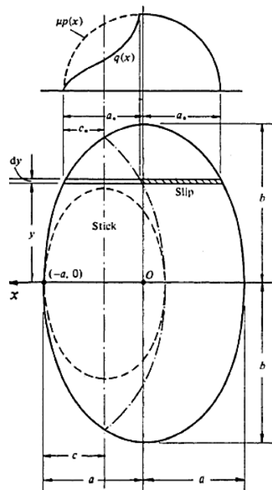
Fig. 5 Contact area based on Vermeulen-Johnson (dashed line) and strip theory (dash-dot line) [8], [11]
