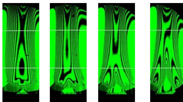
Fig. 10. Fringe maps for different distances between slot nozzles
