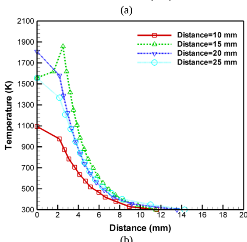
Fig. 11. Temperature profile for different distance between slot nozzles in two sections a) H/D_h = 8 and b) H/D_h = 28
