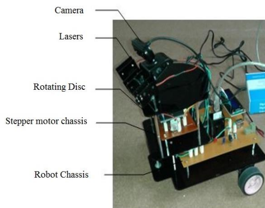
Fig. 2 Architecture of the fabricated mobile robot
