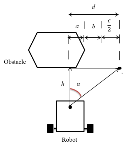
Fig. 6 Parameters of robot path deviation across an obstacle
