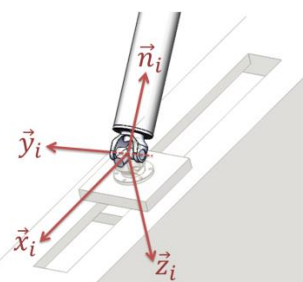
Fig. 6 Axes defined for the universal joint
