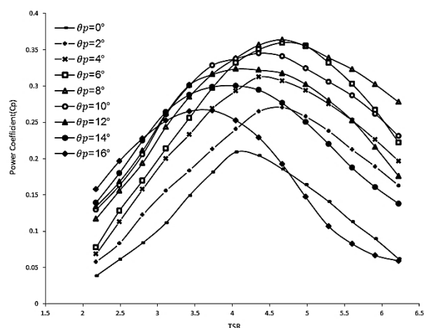
Fig.8 Power Coefficient for different blade pitch angle and chord length 2.2 cm
