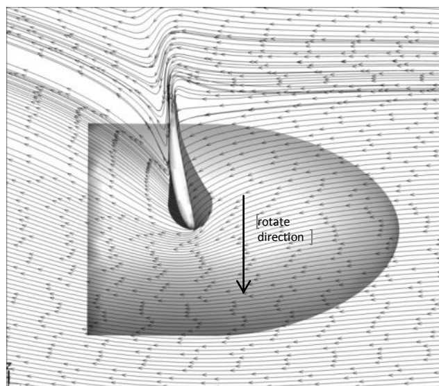
Fig.9 Streamlines for 10° blade pitch angle and 4.97 TSR
