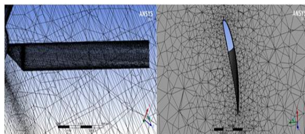
Fig.3 Mesh generated around the blades
