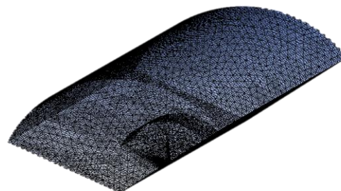
Fig. 2 Computational domain and mesh
