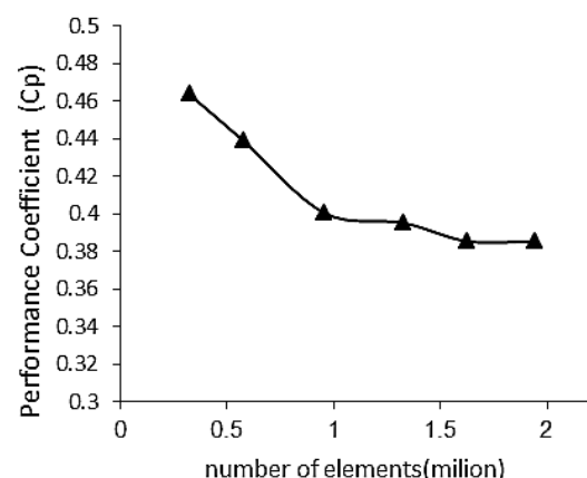
Fig.5 mesh independence
