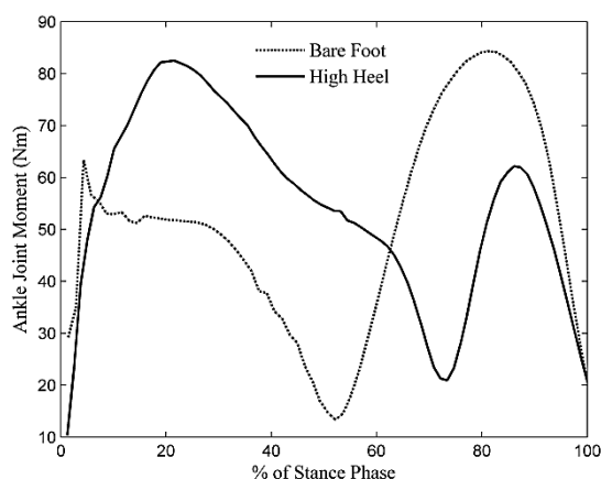
Fig. 14 Diagram of ankle joint moment during stance phase of gait
