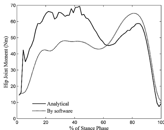
Fig. 18 Diagram of hip joint moment during stance phase of gait
