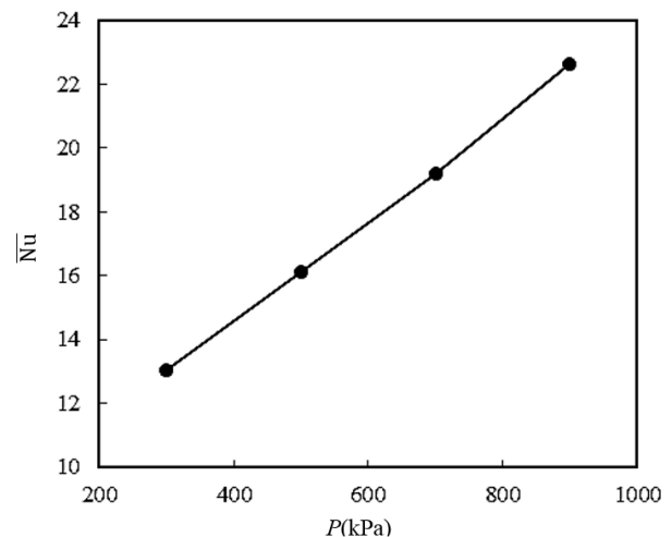
Fig. 6 Average Nusselt number at different angular pressures
