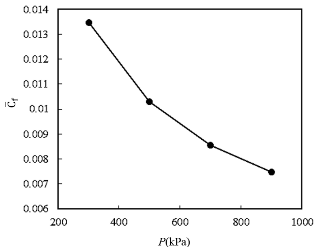
Fig. 7 Average friction coefficient at different angular pressures
