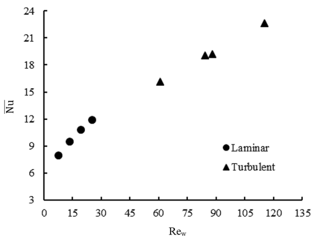
Fig. 8 Average Nusselt number at different kinetic Reynolds
