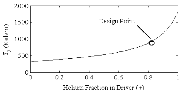
Fig. 6 Required helium fraction in the driver tube as a function of the reservoir stagnation temperature ( T_5 ) for a tailored shock tube operation
