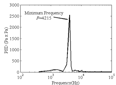
Fig. 14 Acoustic Signal PSD at \theta = 15^\circ
