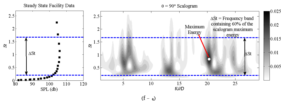
Fig. 11. The scatogram of acoustic pressure signal of the microphones at different polar angles at a) \theta = 15^\circ , b) \theta = 30^\circ c) \theta = 45^\circ d) \theta = 60^\circ , e) \theta = 75^\circ and f) \theta = 90^\circ .
