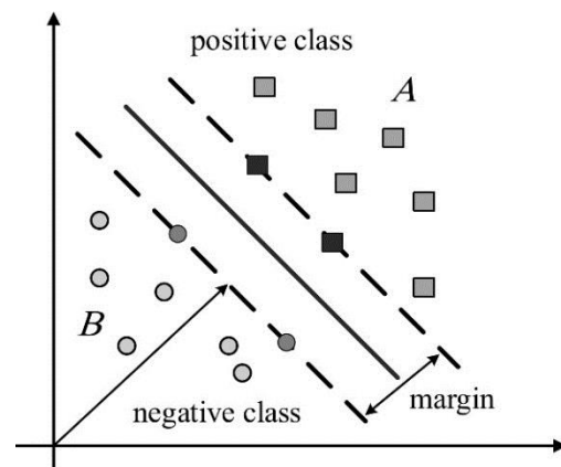
Fig. 1 Data classification using support vector machine.
