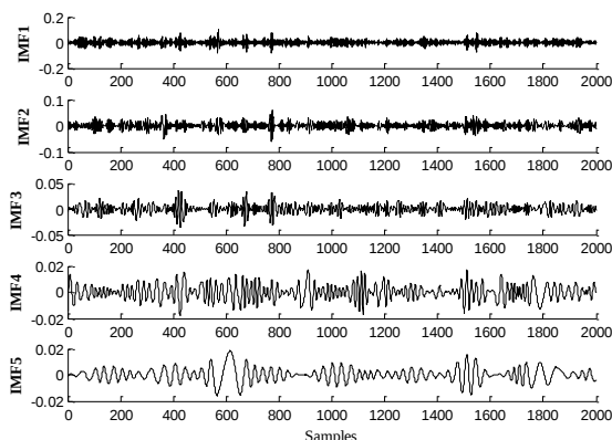
Fig. 4 Decomposition of vibration signal with EMD method
