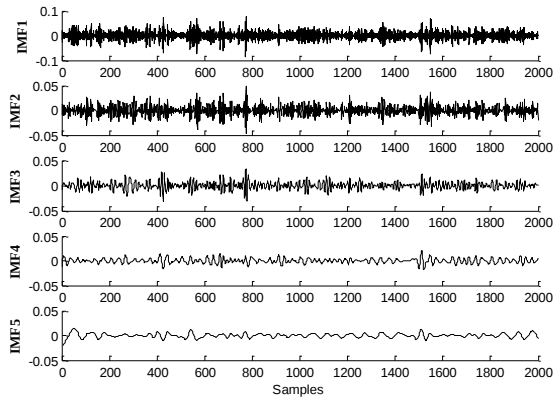
Fig. 5 Decomposition of vibration signal with EEMD method
