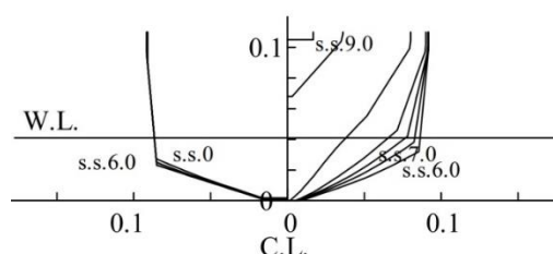
Fig. 5 Body Plan of the Sample Vessel
