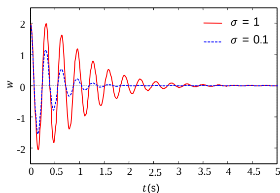
Fig. 11 The Impact of \sigma on the Response Time History at 0.17 Volume Fraction
