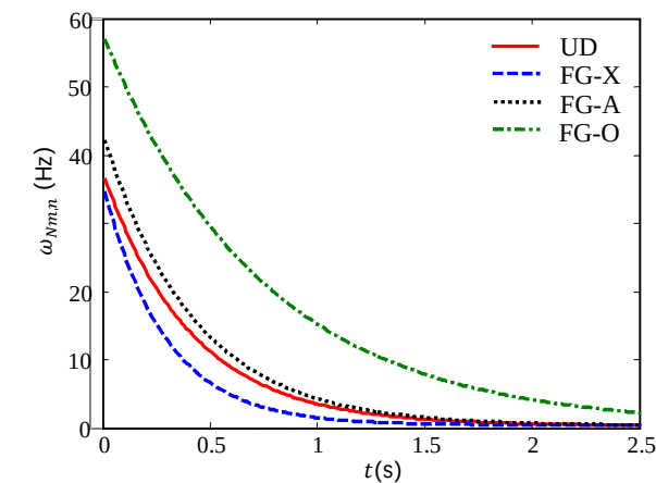
Fig. 4 Normal Nonlinear Frequency Based on Time for Different Distributions of Carbon Nanotubes at 0.12 Volume Fraction
