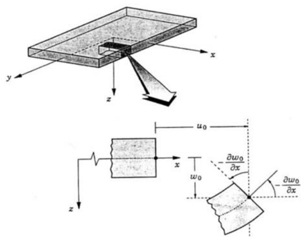
Fig. 1 A Perspective of Movement in the Classic Theory of Plates
