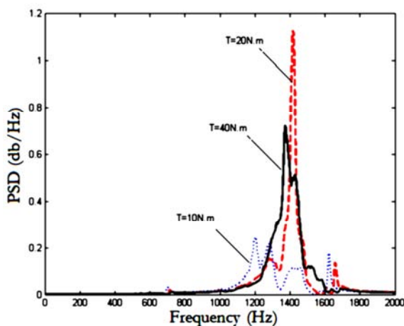
Fig. 6 Power spectral density for different values of connection torques
