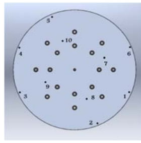
Fig. 5 Vibration sensors arrangement on head expander
