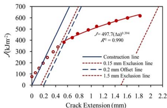
Fig. 10 Experimental J-\Delta a data for base metal
