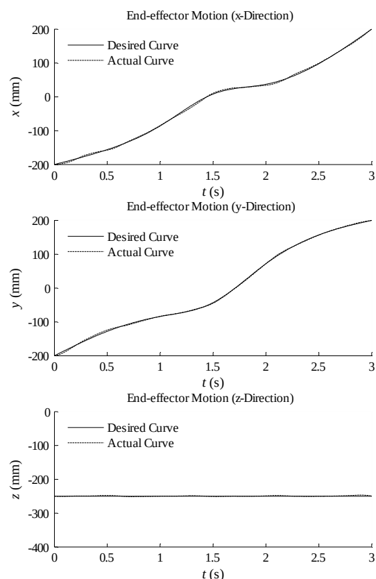
Fig. 10 End-effector motion plots
