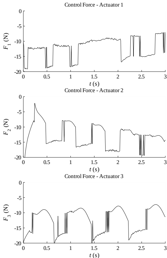
Fig. 13 Control signals
