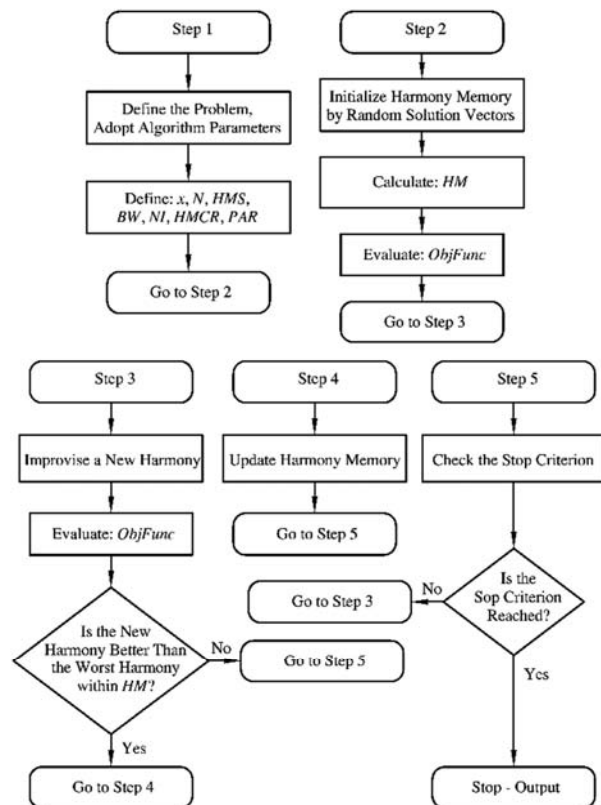
Fig. 4 Flowchart of harmony search algorithm
