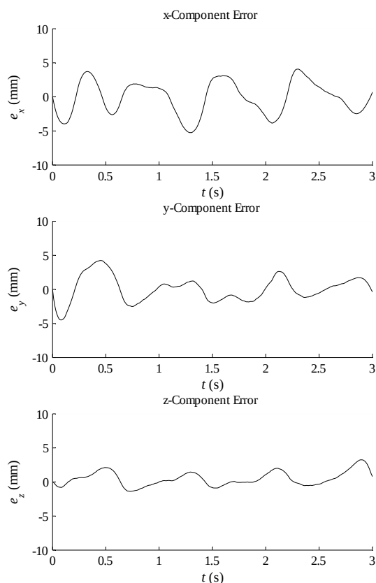
Fig. 12 Tracking-error components
