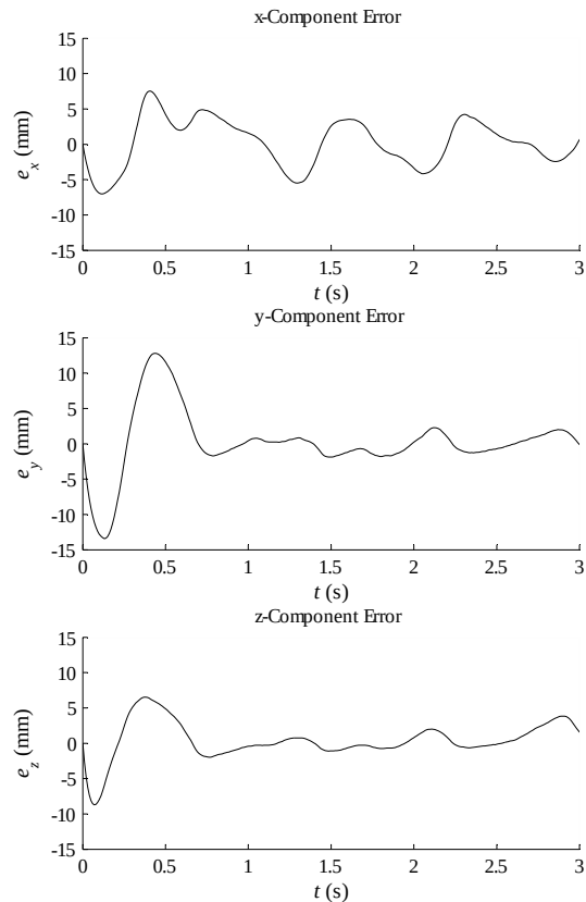
Fig. 21 Error components
