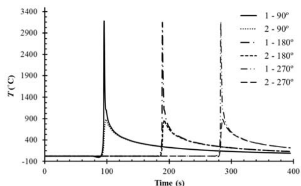
Fig. 13 Temperature versus time in the sixth case welding
