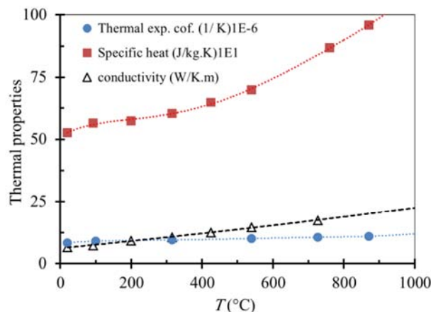
Fig. 2 Thermal properties of titanium alloy (Ti-6Al-4V) at different temperatures [19]
