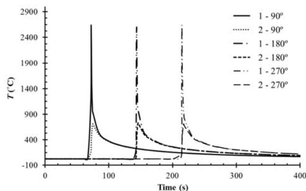
Fig. 10 Temperature versus time in the third case welding
