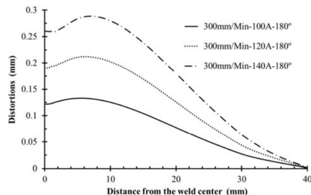
Fig. 30 Distortion in the welding progress speed of 300mm/Min
