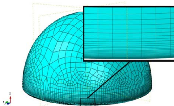
Fig. 3 Model meshing
