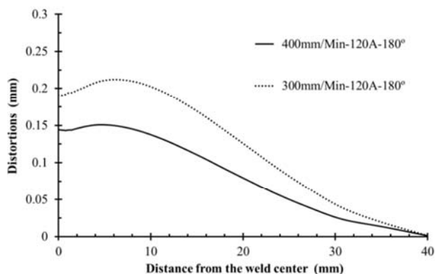
Fig. 32 Distortion in the 120A current
