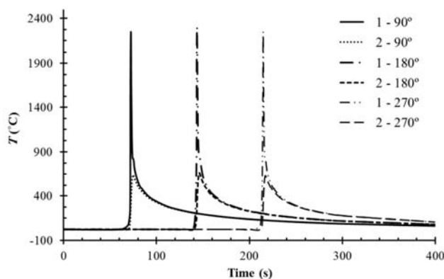
Fig. 9 Temperature versus time in the second case welding
