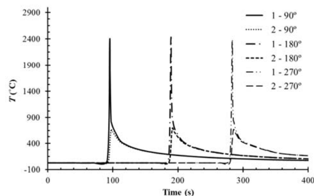
Fig. 11 Temperature versus time in the fourth case welding
