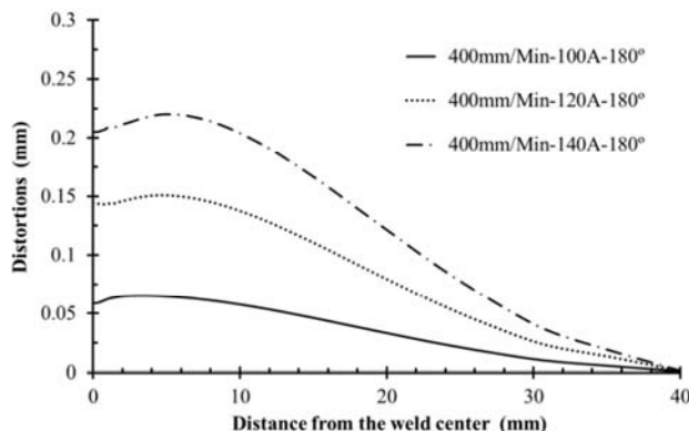
Fig. 29 Distortion in the welding progress speed of 400mm/Min
