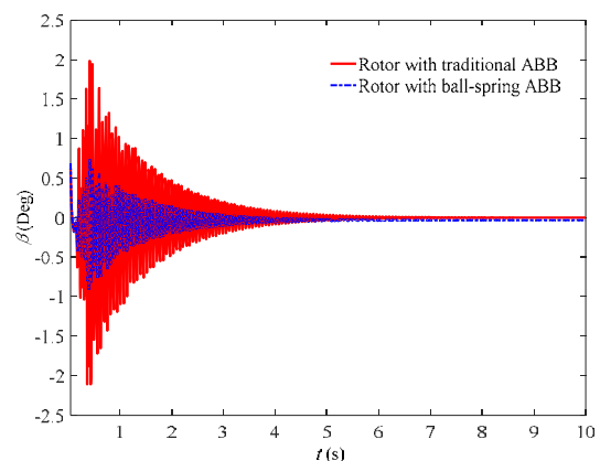
Fig. 10 Time response of Euler angle, \beta
