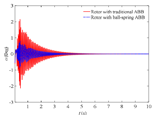
Fig. 9 Time response of Euler angle, \alpha
