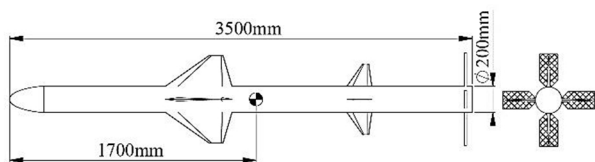
Fig. 11 The general model with Grid fin
