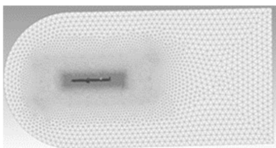
Fig. 18 Mesh quality at the cross-section parallel to the axis
