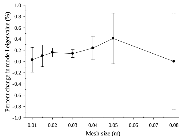
Fig. 6 The percentage of variations mesh dependency between critical buckling mode I and mesh sizes for spheroid shell with h=3\text{mm}
