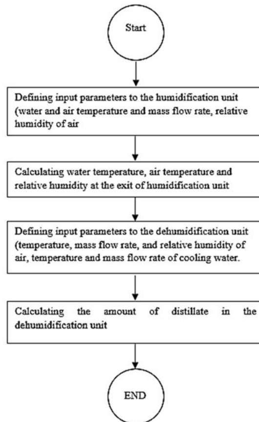
Fig. 3 Flowchart for simulation of the desalination system
