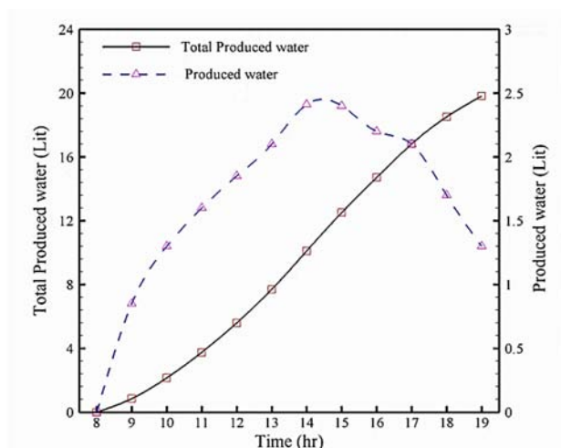
Fig. 5 Hourly and cumulative fresh water produced
