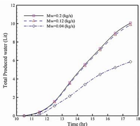
Fig. 12 The cumulative fresh water produced
