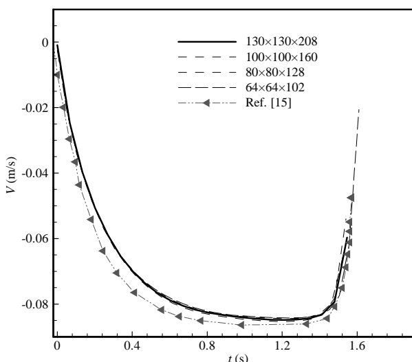
Fig. 10 Grid study for simulation of settling sphere in a quiescent fluid.
