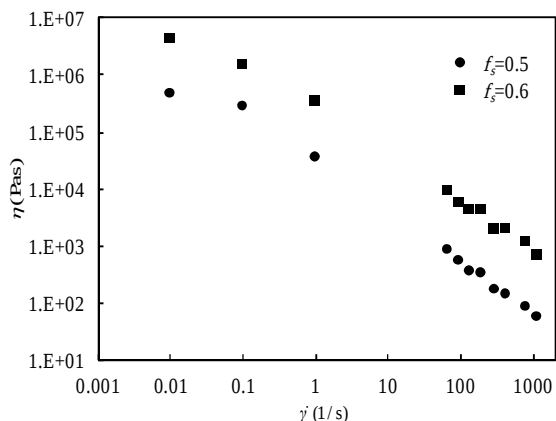
Fig. 7 Viscosity changes over a wide range of shear rates
