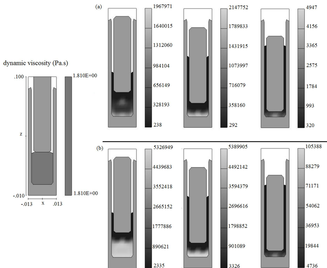
Fig. 13 Viscosity contours in different time frames for (a) f_s=0.5 , R_p=8\text{mm} , V_r=100\text{mm/s} and (b) f_s=0.6 , R_p=8\text{mm} , V_r=70\text{mm/s}
