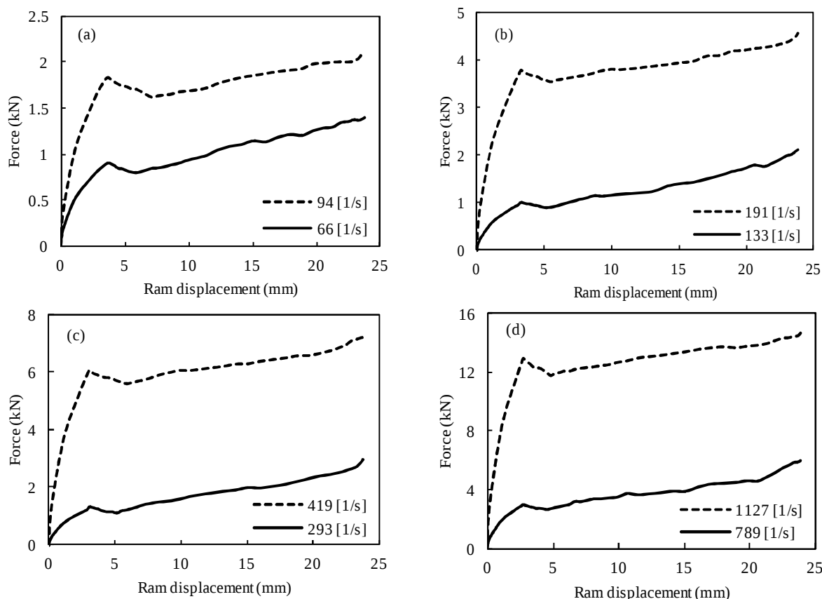
Fig. 6 Variations of force versus ram displacement at 0.6% solid fraction and punch diameters: a-15mm, b-16mm, c-17mm, d-18 mm
