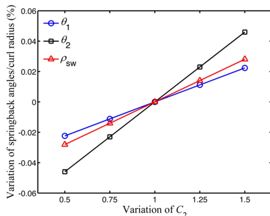
Fig. 17 Influence of C_2 variation on the springback parameters
