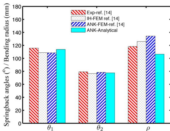
Fig. 14 Comparison of several experimental and theoretical predictions of the springback parameters based on FEM method and analytical method
