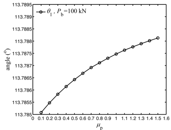
Fig. 11 Effect of the punch friction coefficient on the angle \theta_1
