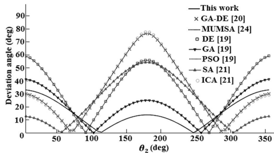
Fig. 7 Deviation of transmission angle from 90°
