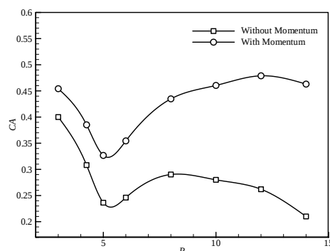
Fig. 10 The axial force coefficient of Case 5 versus P at zero angle of attack and D=7.6
