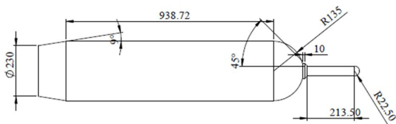
Fig. 1 Dmension of the spiked blunt body [6]
