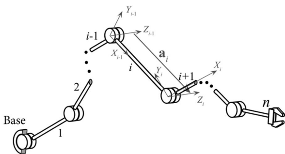
Fig. 1 3D Schematic representation of an nR -PSM
