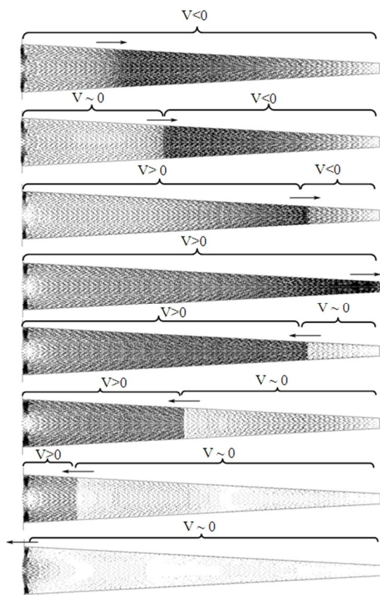
Fig. 10 Axial velocity vectors inside the tube during cycle change
