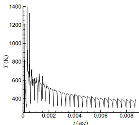
Fig. 8 Numerical results of temperature data vs. time for the extracted gas at point P_4 for case 3
