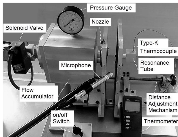
Fig. 2 Schematic view of Hartmann-Sprenger device test stand
