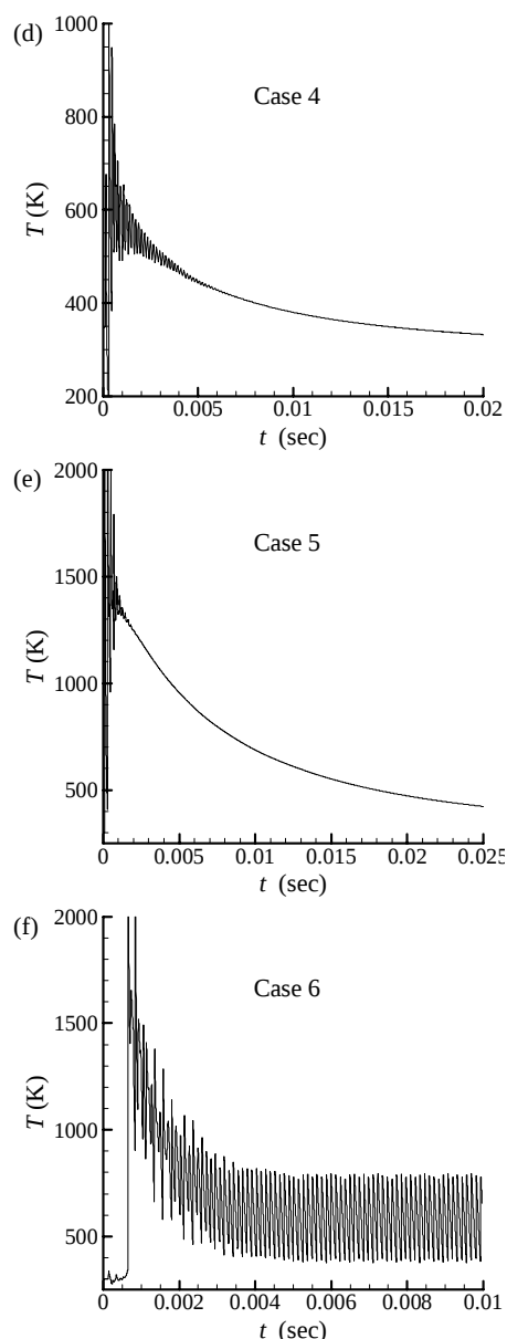
Fig. 7 Numerical results for temperature data at point P_3
