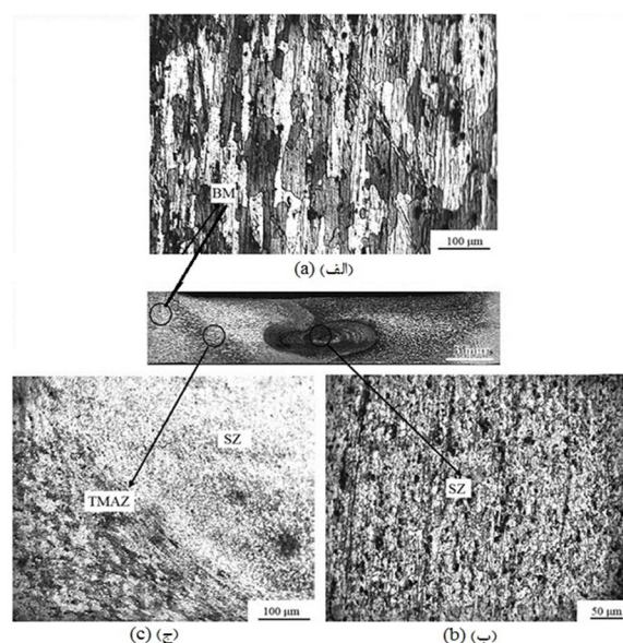
Fig. 6 Micrograph is showing cross section nanocomposite (a) BM (b) SZ (c) TMAZ
