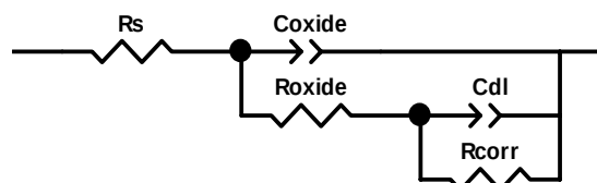
Fig. 6 Equivalent circuit for fitting impedance diagrams
