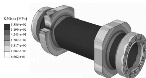
Fig. 9 Von Mises Stress distribution on gas generator's mass-launcher
