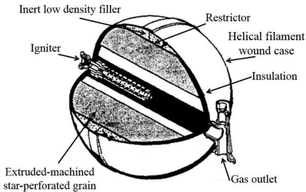
Fig. 1 Spherical gas generator [13]
