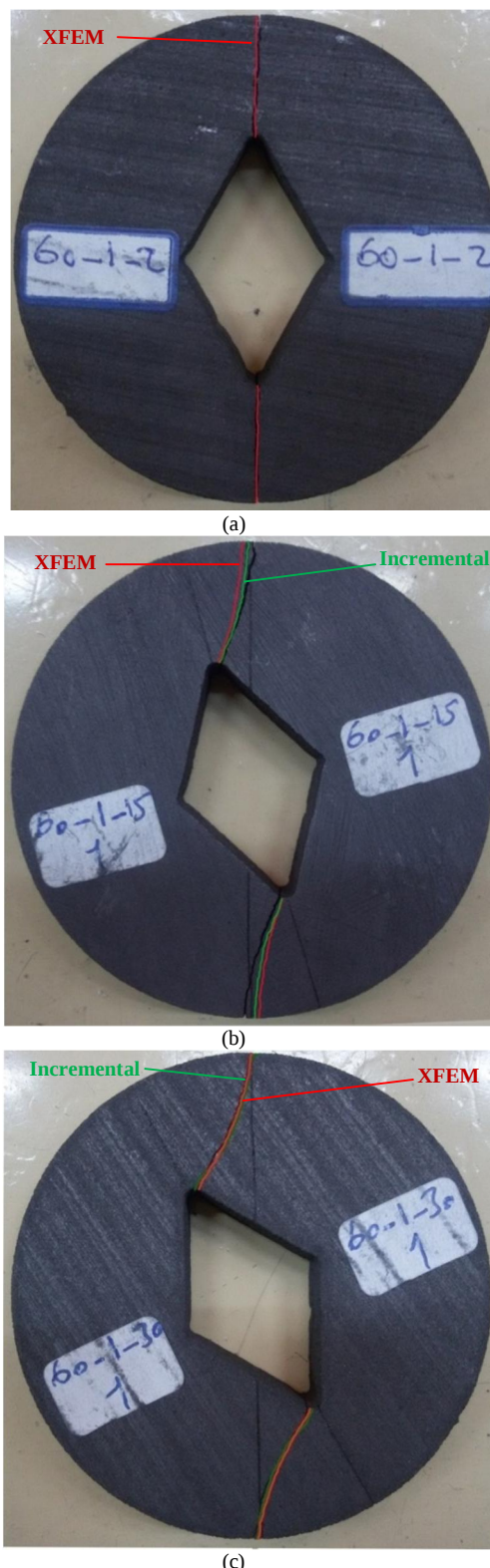
Fig. 10 The fracture trajectory of RV-BD with 2\alpha=60^\circ under a) pure mode I ( \beta=0^\circ ), b) mixed mode I/II ( \beta=15^\circ ), c) pure mode II loading ( \beta=30^\circ ) obtained from XFEM, incremental method and experiments.
