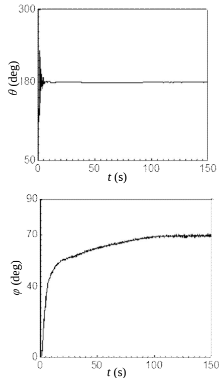
Fig. 16 Module positioning for \theta_d=180^\circ and \varphi_d=70^\circ with 5 V activation voltage (a) \theta , (b) \varphi
