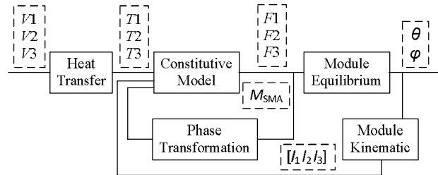
Fig. 6 Block diagram of module numerical simulation
