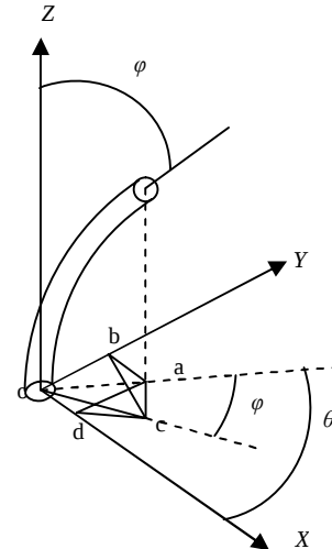
Fig. 5 Relation of \theta and \varphi angles with inclination of end plate
