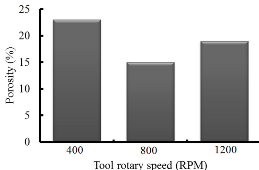
Fig. 20 Porosity changes with tool rotary speed
