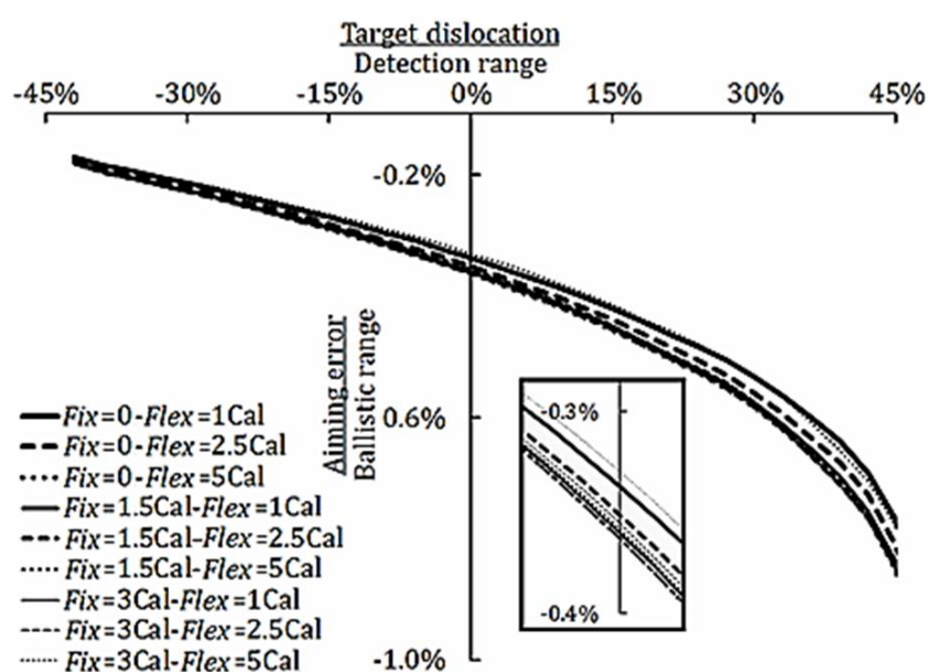
Fig. 8 Impact error of nine missiles, fired at angle of 30^\circ
