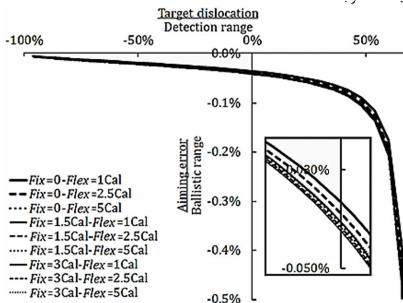
Fig. 12 Geometry effect on permanent thrust missile aiming error, fired at angle of 30^\circ
