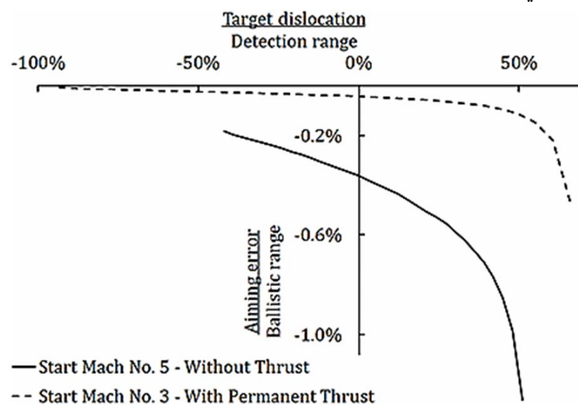
Fig. 11 Thrust effect on improving the accuracy of surface to surface missile, fired at angle of 30^\circ
