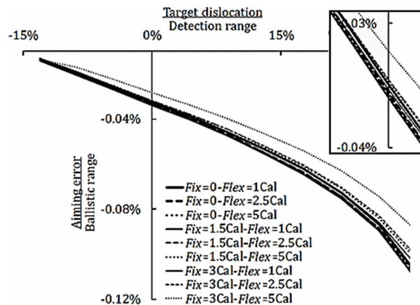
Fig. 9 Impact error of nine missiles, fired at angle of 80^\circ
