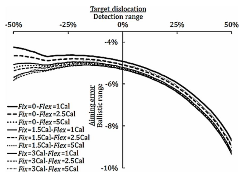
Fig. 10 Impact error of nine missiles, fired at angle of 10^\circ
