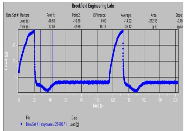
Fig 1 Texture profile analysis measurement of mayonnaise with 25% reduced fat and containing 100 ppm nanoemulsions of Cordia myxal fruit extract
