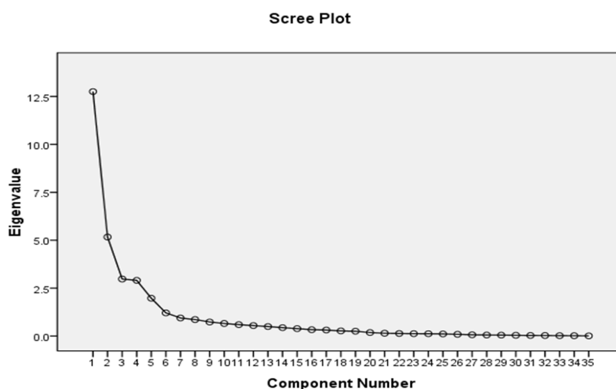
Figure 1: Scree plot.
