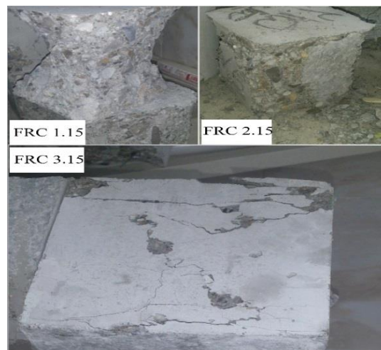
Fig. 4. Specimens containing 0.15% PET fiber after compressive test
