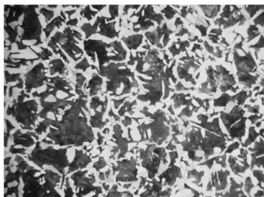
Fig. 6 Steel (1.1191) with Microstructure of Ferrite-Perlite
