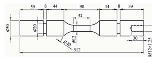
Fig. 8 The Final dimension of Tension specimen
