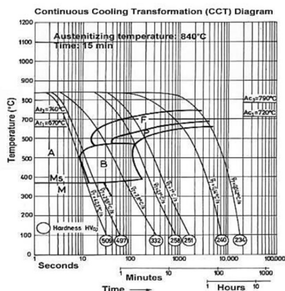
Fig. 1 Time-Temperature Transformation Diagram of 1.1191 [7]
