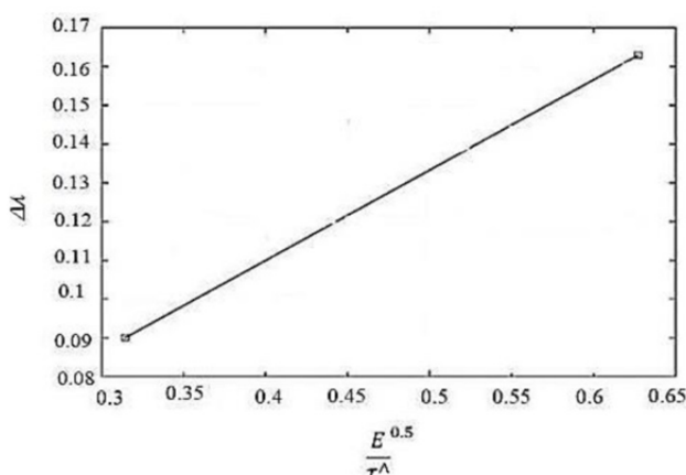
Fig. 16 Dependence of stress ratio on acoustic softening density of 1.1191 (ferrite-perlite)
