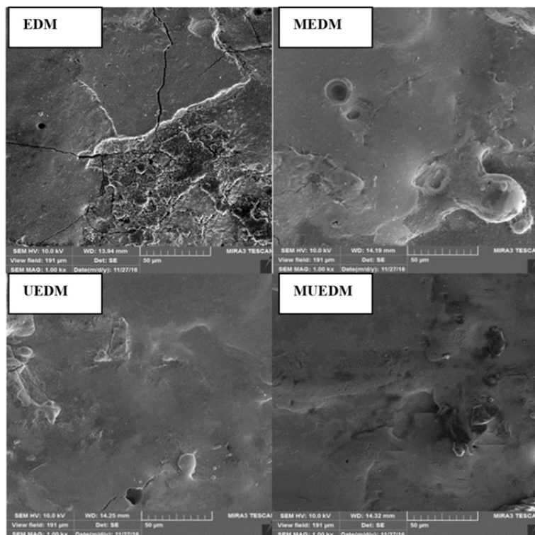
Fig. 8 The SEM picture of machined surfaces in I=32 A, T_{on}=12.8 \mu s with (a) EDM (b) MEDM (c) UEDM, and (d) MUEDM processes
