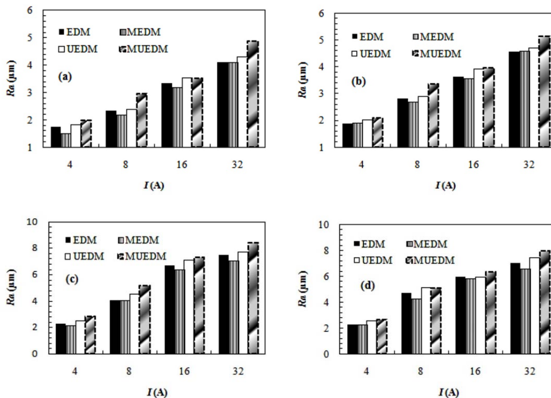
Fig. 3 Effects of pulse current on surface roughness of MUEDEM as compared with EDM, MEDM and UEDM processes at (a) T_{on}=6.4 \mu s (b) T_{on}=12.8 \mu s (c) T_{on}=50 \mu s (d) T_{on}=100 \mu s
