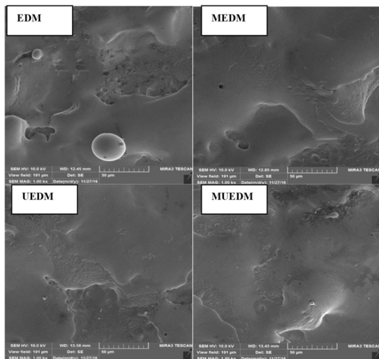
Fig. 7 The SEM picture of machined surfaces in I=8 A, T_{on}=50 \mu s with (a) EDM (b) MEDM (c) UEDM, and (d) MUEDM processes
