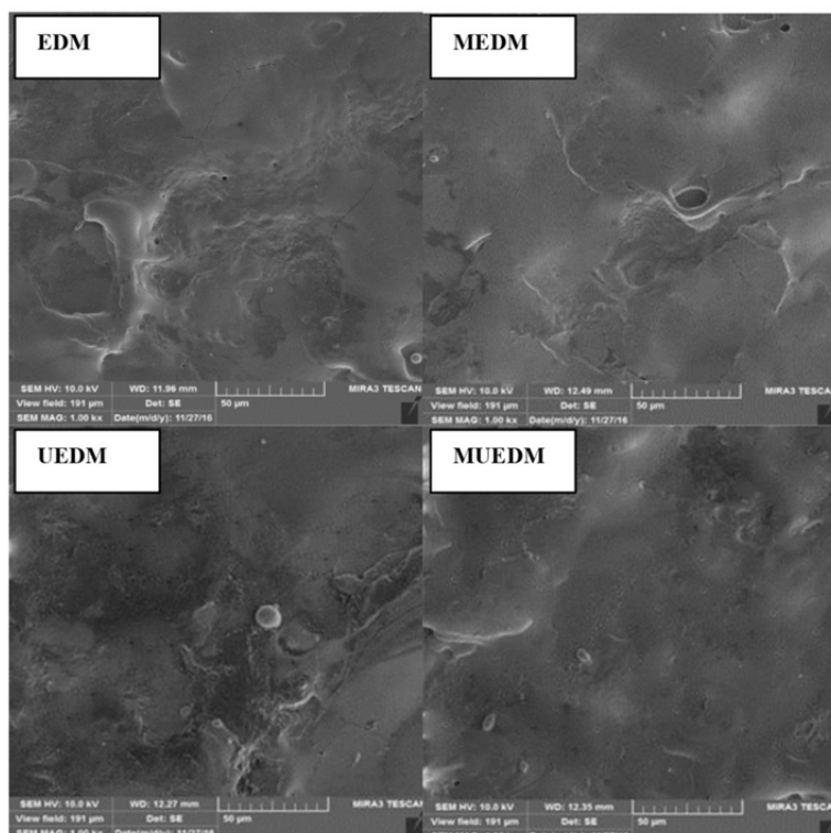
Fig. 9 The SEM picture of machined surfaces in I=8 A, T_{on}=12.8 \mu s with (a) EDM (b) MEDM (c) UEDM, and (d) MUEDM processes
