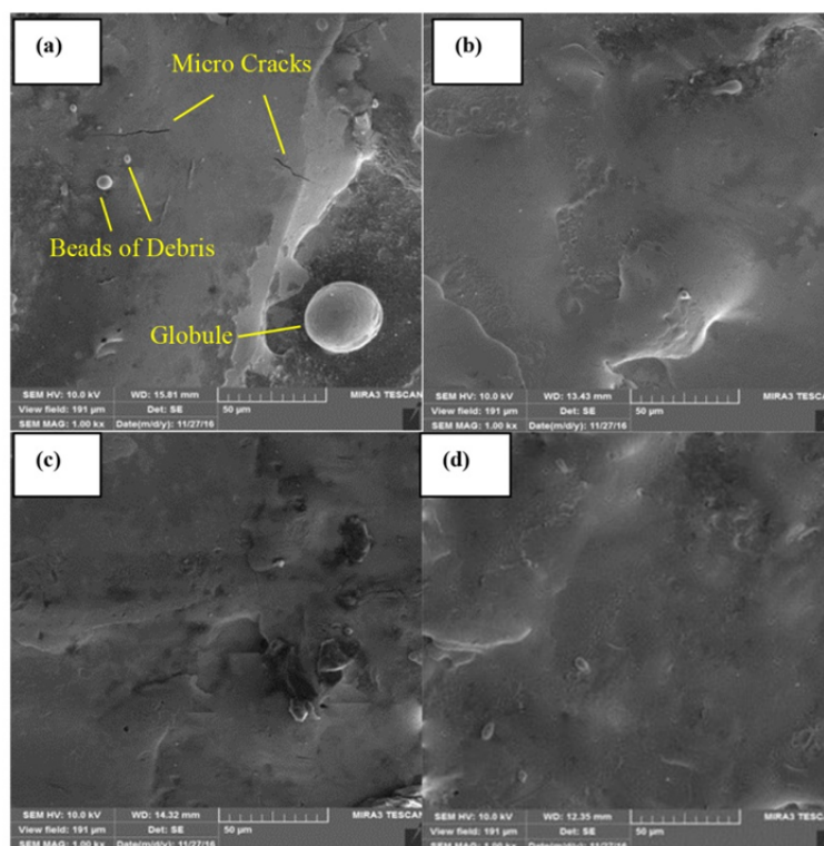
Fig. 5 The SEM picture of machined surfaces with MUEDM process in different pulse currents and pulse durations (a) 32 A, 50 \mu\text{s} (b) 8 A, 50 \mu\text{s} (c) 32 A, 12.8 \mu\text{s} (d) 8 A, 12.8 \mu\text{s}
