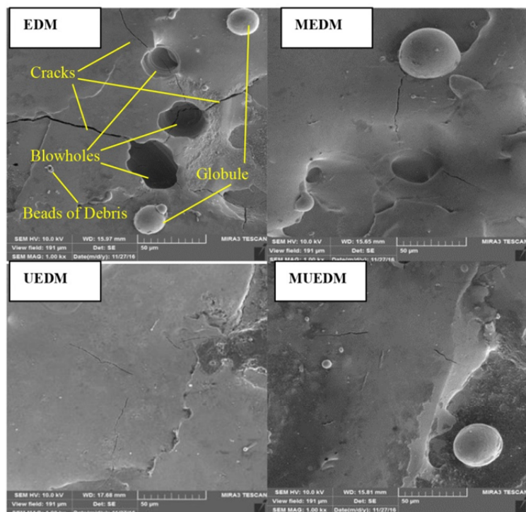
Fig. 6 The SEM picture of machined surfaces in I=32 A, T_{on}=50 \mu s with (a) EDM (b) MEDM (c) UEDM, and (d) MUEDM processes
