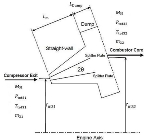
Fig. 2 Diffuser model and input and output parameters [10]
