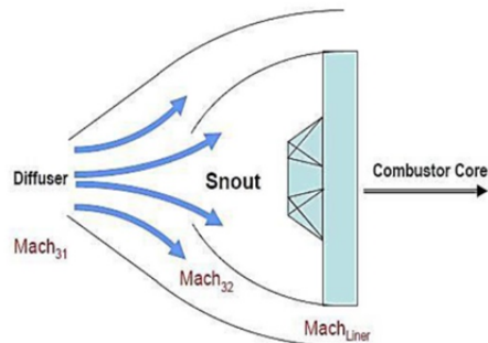
Fig. 3 Snout section located between the diffuser and liner [9]
