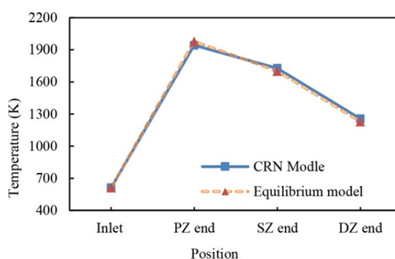
Fig. 10 The CFM-56 axial temperature variations across combustor zones for approach condition
