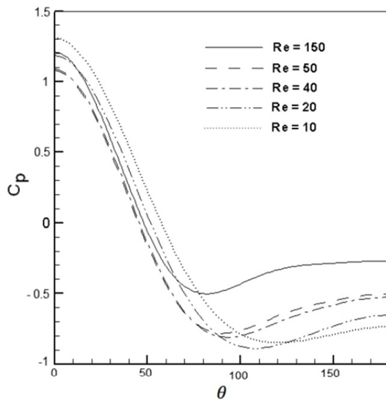
Fig. 13 Pressure coefficient for different Reynolds number on 80×80 uniform grid
