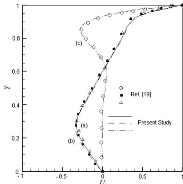
Fig. 7 Comparison of u -velocity profiles along vertical centerline at Re = 400 and (a) Gr = 10^2 , (b) Gr = 10^4 , (c) Gr = 10^6 on 80 \times 80 uniform grid
