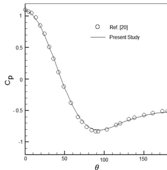
Fig. 12 Comparison of pressure coefficient at Re = 40
