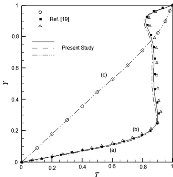
Fig. 6 Comparison of results for temperature profiles along vertical centerline at Re = 400 and (a) Gr = 10^2 , (b) Gr = 10^4 , (c) Gr = 10^6 on 80 \times 80 uniform grid
