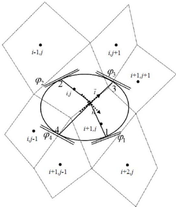
Fig. 3 Proposed stencil for evaluating convective fluxes
