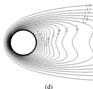
Fig. 14 Computed isotherms at (a) Re = 10 , (b) Re = 20 , (c) Re = 40 and (d) Re = 50 on 80 \times 80 uniform grid
