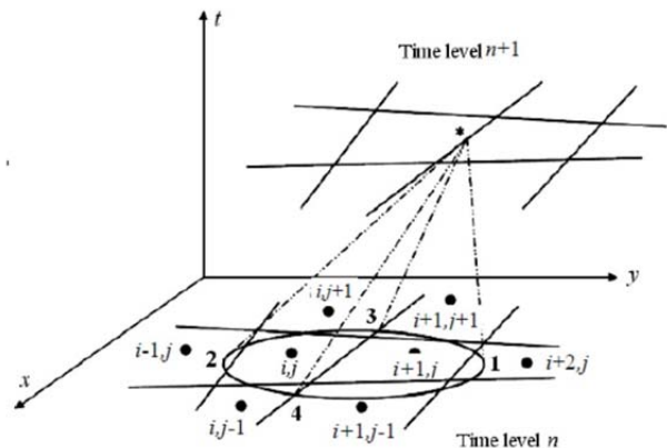
Fig. 2 Intersection of local Mach cone with time level plane
