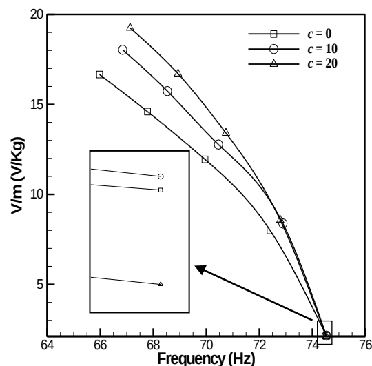
Fig. 10 Backbone curve, L=68\text{mm}
