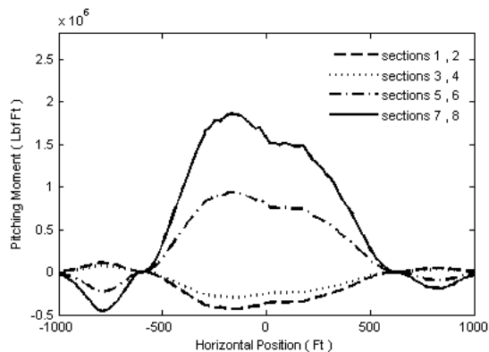
Fig. 9 The pitching moment induced by the wind effect to per section vs. location of microburst.
