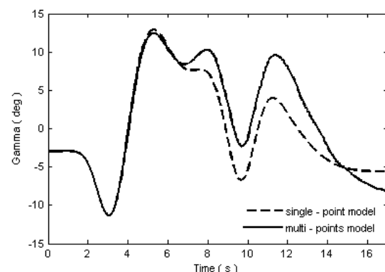
Fig. 16 The heading angle graph for the both models
