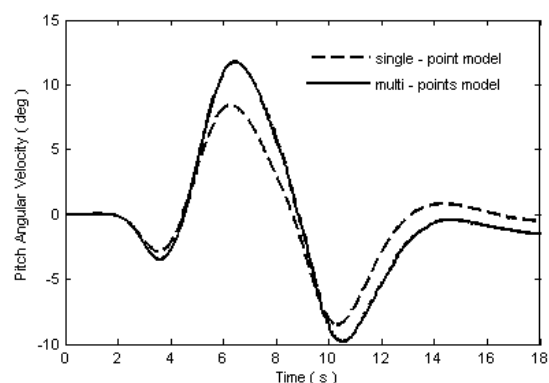
Fig. 14 The angular velocity (q) graph for the both models
