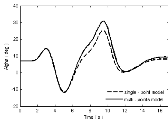
Fig. 15 The angle of attack graph for the both models
