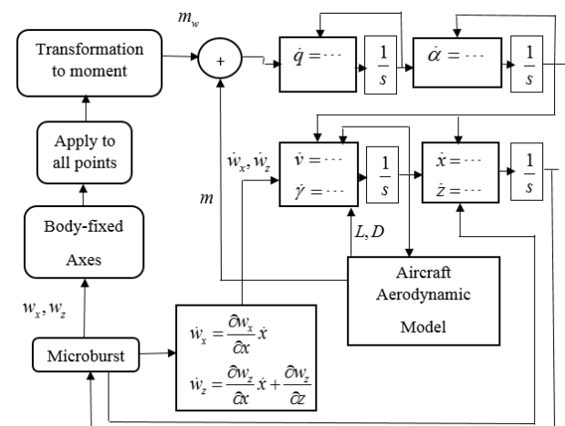
Fig. 5 Schematics of the aircraft multi-points model equations under the microburst influence
