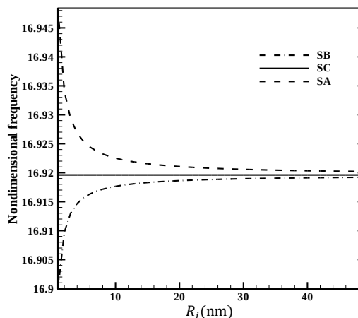
Fig. 4 Second dimensionless torsional natural frequencies for n = 3 , R_o/R_i = 1.1 and three surface types
