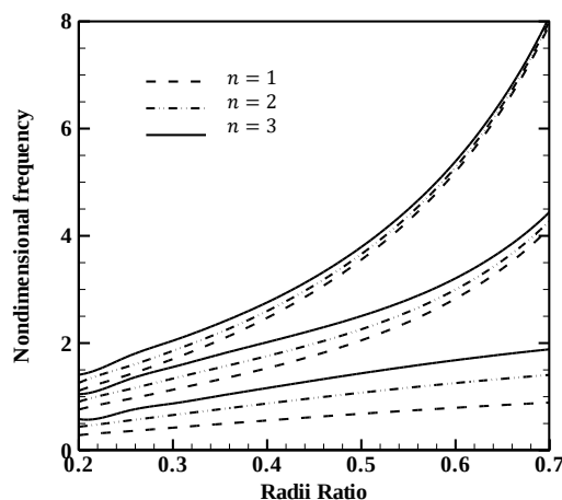
Fig. 11 dimensionless torsional natural frequencies versus R_i/R_o for R_o = 2 nm and SB surface
