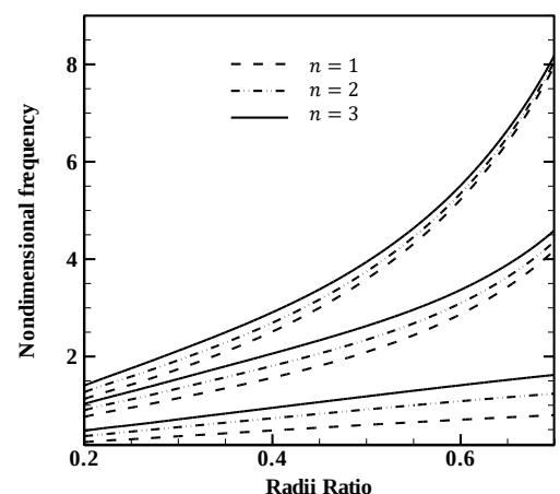
Fig. 12 dimensionless torsional natural frequencies versus R_i/R_o for R_o = 2 nm and SA surface
