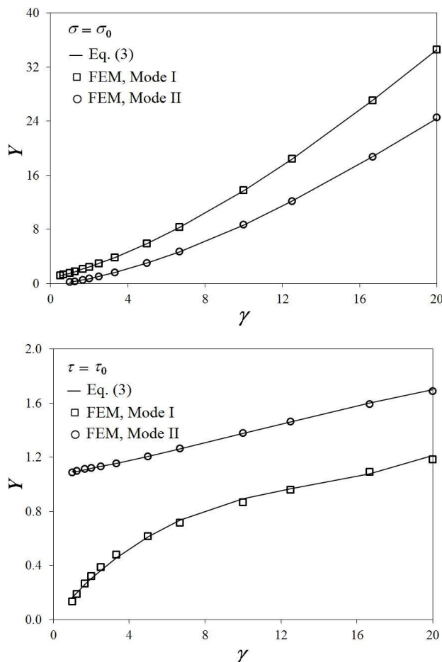
Fig. 9 Fitting of third-degree of polynomial on the geometry correction factors of subsurface crack under uniform tension and shear
