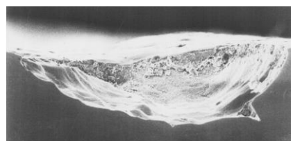
Fig. 1 Pitting of the contact surface due to a subsurface crack growth
