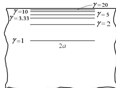
Fig. 6 Real scale representation of the proximity to the surface for the studied subsurface cracks
