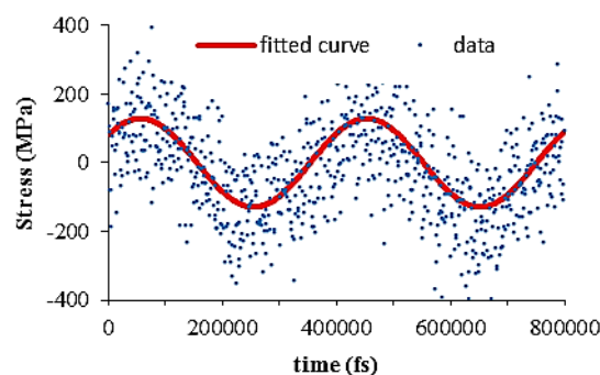
Fig. 7 Calculated stress (points) for applied strain with 2.5 GHz frequency to the PVDF cell obtained from DMA in tensile mode and the fitted curve
