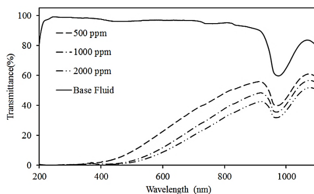
Fig. 4 Transmittance of silica nanofluids at different wavelengths
