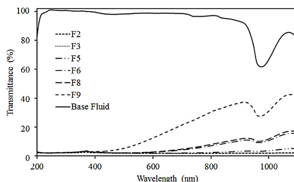
Fig. 5 Transmittance of hybrid nanofluids at different wavelengths
