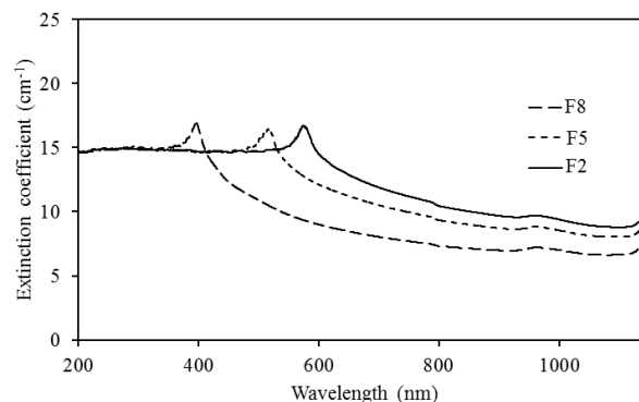
Fig. 6 Extinction coefficient of hybrid nanofluids at different wavelengths
