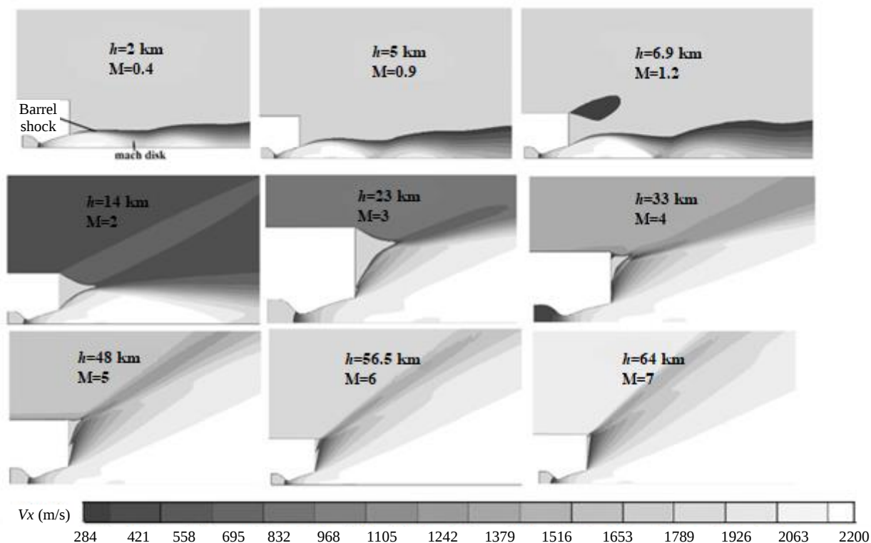
Fig. 7 Velocity contours in the missile exit at different Mach numbers (m/s)
