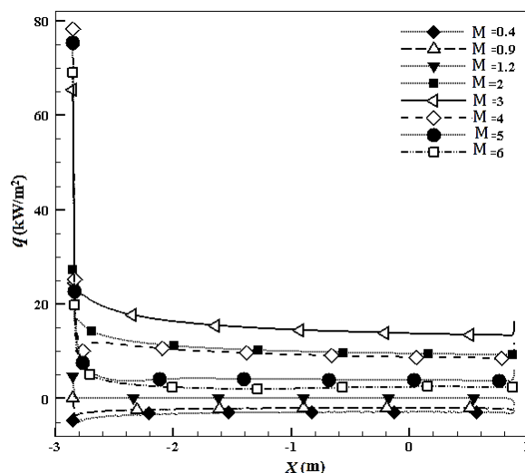
Fig. 9 Heat flux variations of missile body at different Mach numbers
