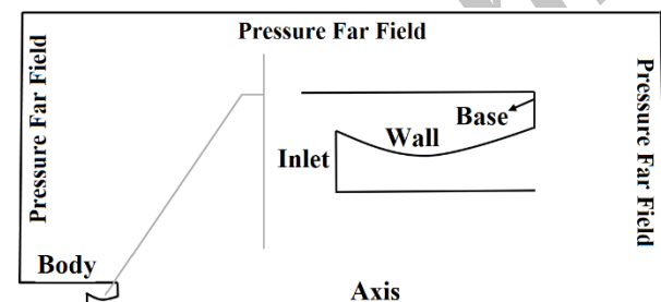
Fig. 3 Schematic of the problem
