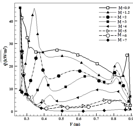
Fig. 10 Heat flux variations of missile base at different Mach numbers
