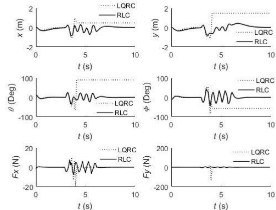
a) The response of the system to the non-impact force in the x and y directions
